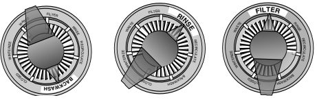
Fig. 9: Valve settings for startup. Stop pump before changing valve position.
